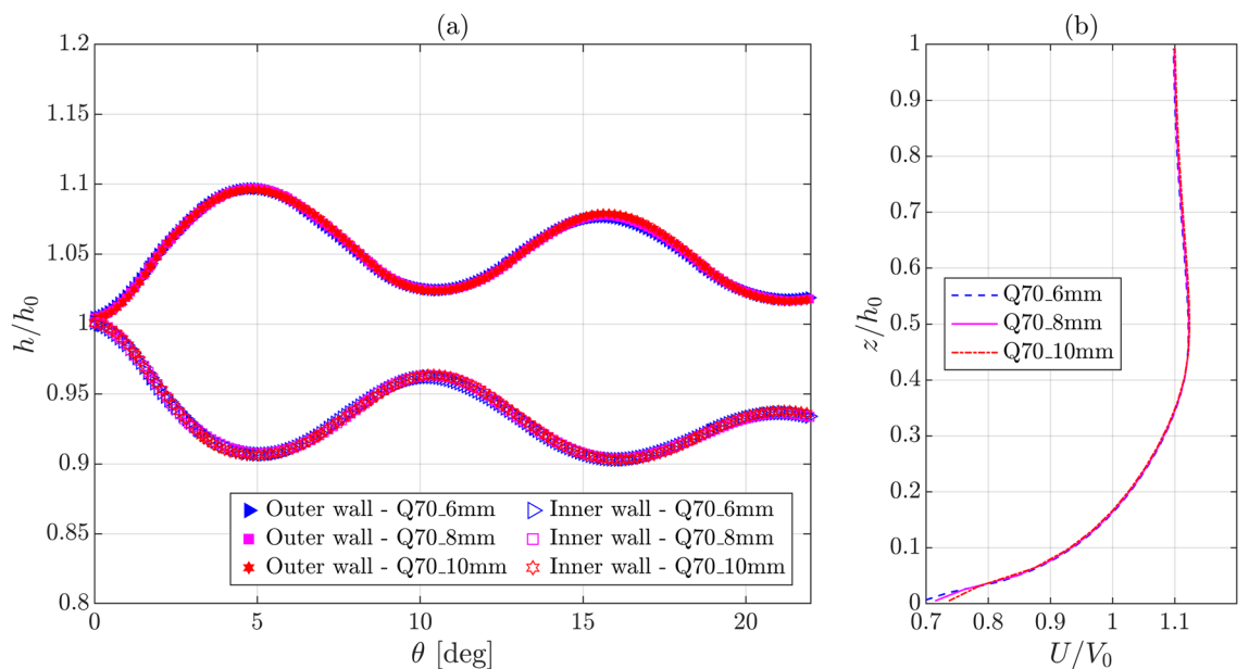
Figure 4. Comparison among the numerical results obtained for different grid arrangements at Q=0.07 \text{ m}^3/\text{s} : (a) normalized WSPs along the outer and inner walls and (b) normalized longitudinal velocity profiles at the channel center located on the bend entrance plane [Q70_8mm is also used as case name Q70; see Table 2 for the legend details].
