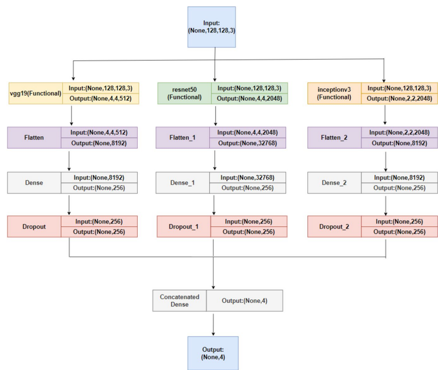
Figure 8. Architectural diagram of layers of ensembled model.
