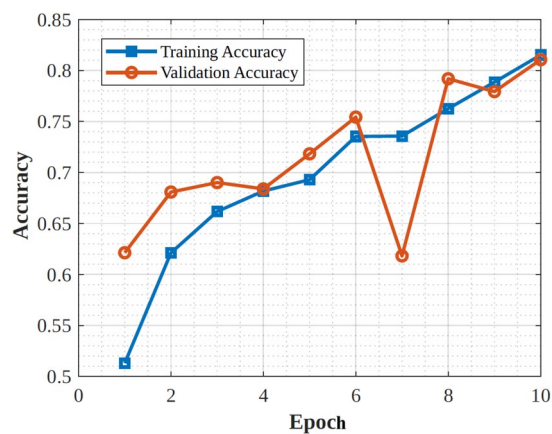
Figure 18. Ensemble model training and validation accuracy.
