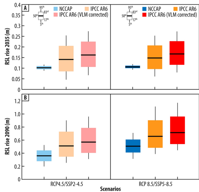
Fig. 5. Comparison of projections of relative sea-level (RSL) rise from the Spanish National Climate Change Adaptation Plan (NCCAP) and IPCC AR6. Projected likely (17–83rd percentiles) and very likely (5–95th percentiles) RSL rise from the NCCAP under RCP4.5 and RCP8.5 scenarios by 2026–2045 and by 2081–2100, compared with the IPCC AR6 sea-level projections under SSP2-4.5 and SSP5-8.5 scenarios by (A) 2035 and (B) 2090, respectively. The IPCC AR6 projections with the updated VLM rate of -0.88 \pm 0.03 mm/yr are also presented. The difference in the projected magnitude of sea-level rise (50th percentile value) are summarized in Table 2. We have standardized the Spanish NCCAP projection to the same baseline as IPCC AR6 of 1995–2014 following ref. 55 .
