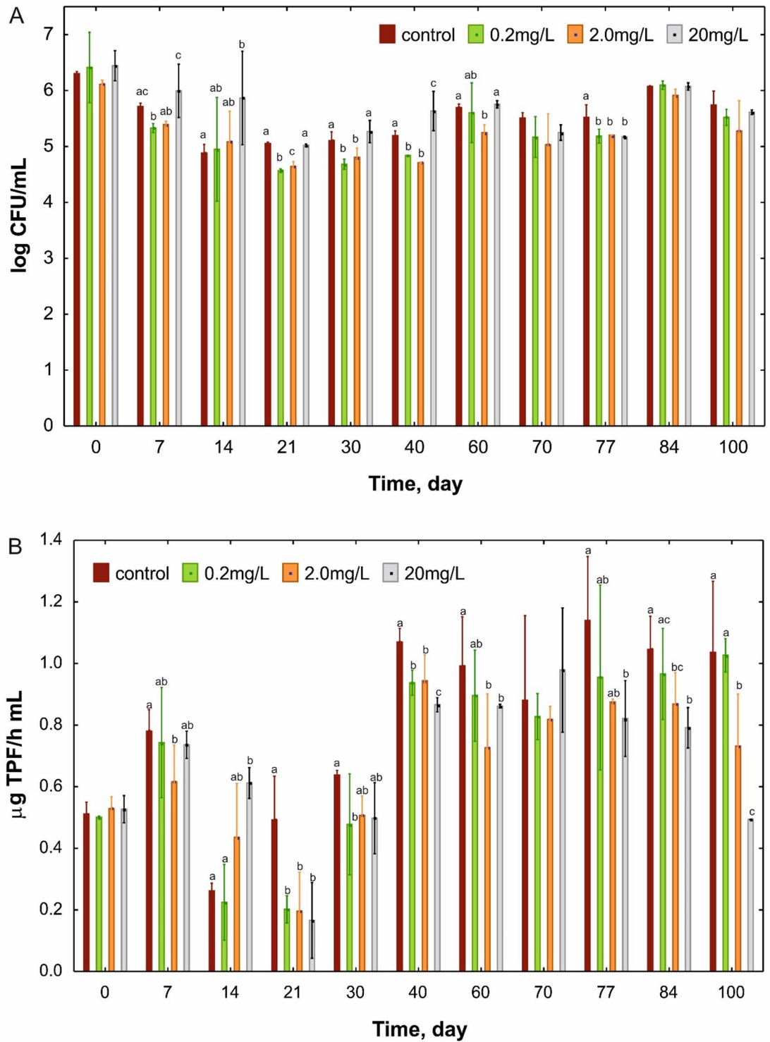
Fig. 2. The number of THB (A) and changes in the TPF (1,2,3-triphenyltetrazolium chloride) concentration (µg/h·mL) (B) in the activated sludge exposed for 100 days to different concentrations of diatrizoate (DTZ). The means with different letters in each sampling day are significantly different ( p < 0.05 , LSD test) considering the effect of DTZ concentration. The means without any letters did not differ among others on the adequate sampling day.
