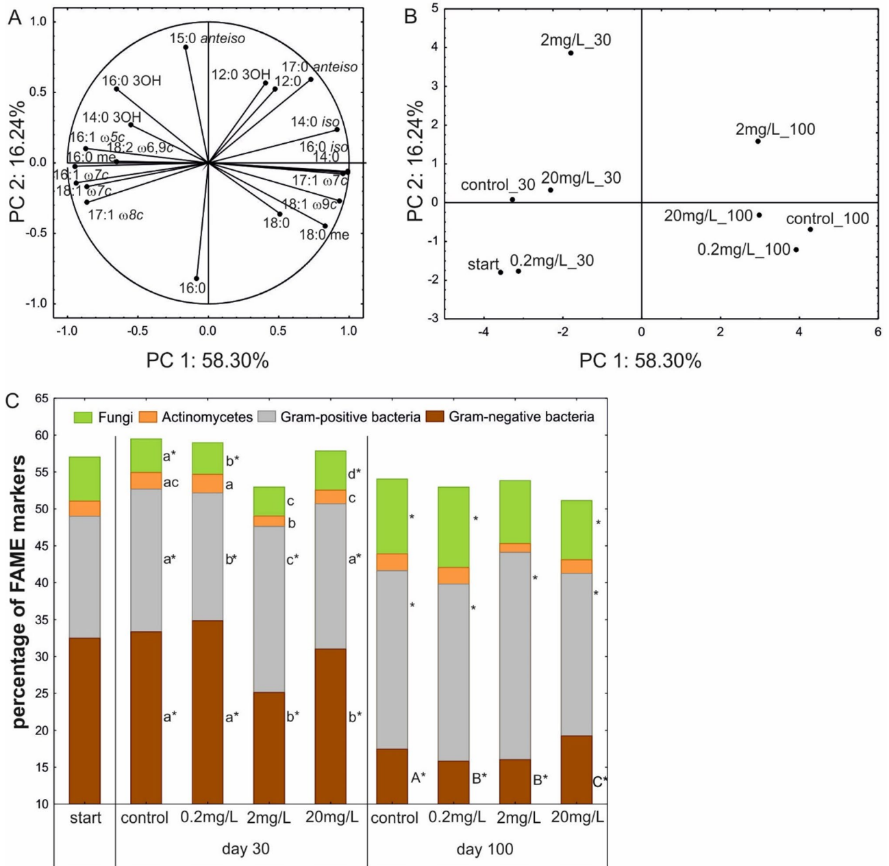
Fig. 4. Projection of fatty acids along PC1 and PC2 (A) and FAME profiles of the control and treated AS (B). The percentages of distinct FAME markers for the control AS and AS treated with DTZ (C). The profile captions X_Y - X - DTZ concentration, Y- sampling day. The means of each FAMEs marker with different letters are significantly different ( p < 0.05 , LSD test) considering the effect of DTZ concentration on the 30th day (lowercase letters) or the 100th day (higher case letters). The means without any letters did not differ among others on the adequate sampling day. The pairs of means with the same concentration of DTZ marked with an asterisk are significantly different ( p < 0.05 , the independent samples t-test) considering the effect of time (30 vs. 100 day).
