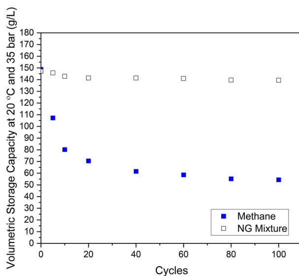
Fig. 3. Deterioration of natural gas storage capacities with successive cycling.
