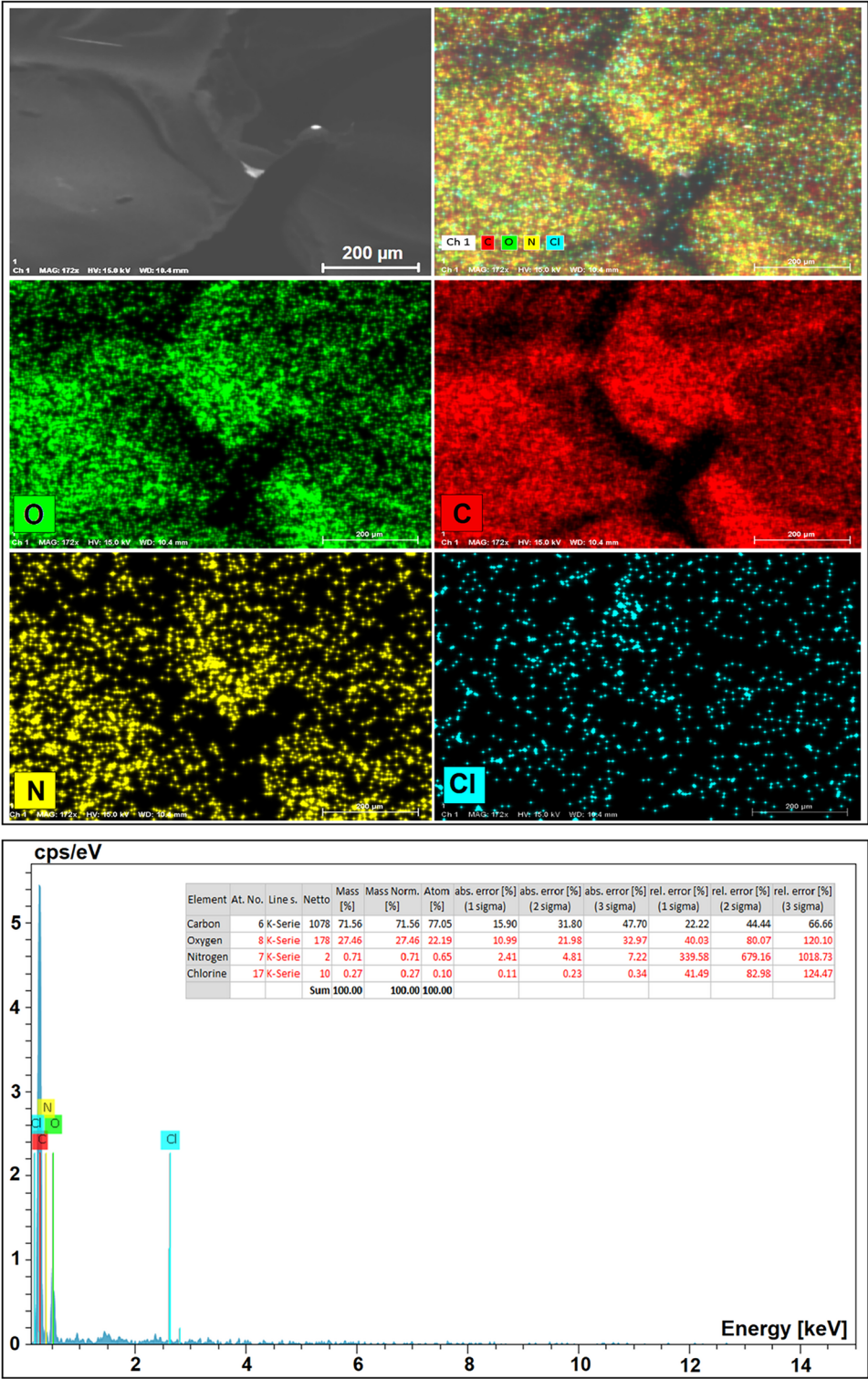
Fig. 7. The result of the X-ray map and EDX analysis for the Cl-DMH-PUSF sample.
