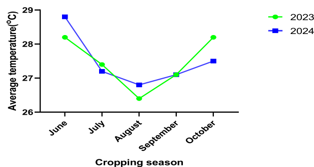
Fig. 3. Temperature distribution in the 2023 and 2024 seasons.
