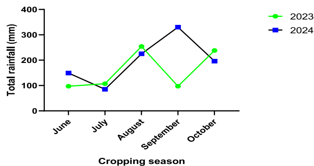
Fig. 2. Total rainfall distribution in the 2023 and 2024 seasons.
