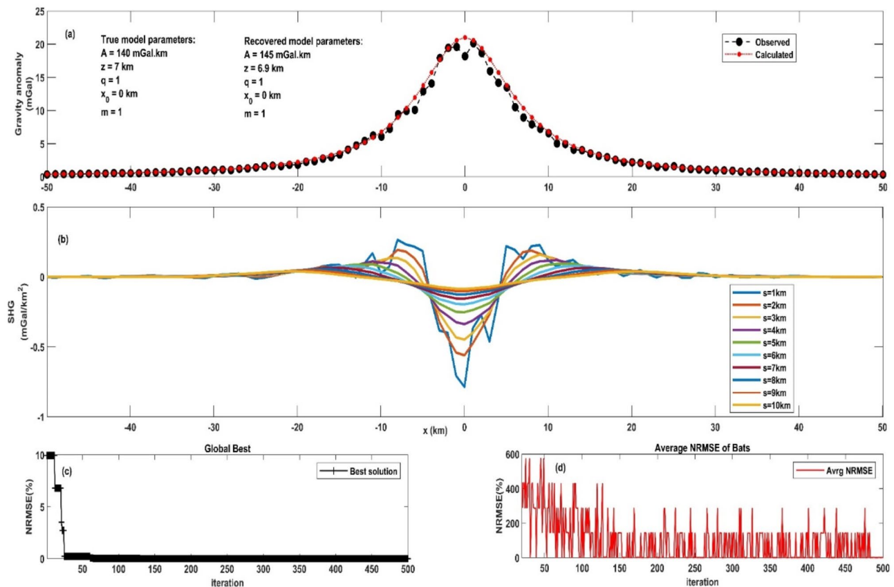
Fig. 5. First model, a horizontal cylinder, in case of a 5% noise level condition. Panel (a) exhibits the observed gravity anomaly profile (illustrated by black circles) alongside the computed optimal gravity response (depicted by red circles) employing the MBA algorithm technique. Panel (b) demonstrates the SHG anomalies using varying ‘s’ window values. Panel (c) depicts the NRMSE of the global optimum solution ( F_{Obj} ) of the bats relative to the number of iterations. Panel (d) shows the average NRMSE of all the bats.
