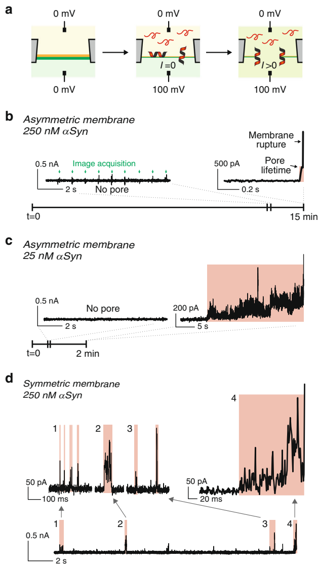
Fig. 2 αSyn pore formation on asymmetric and symmetric membranes.
