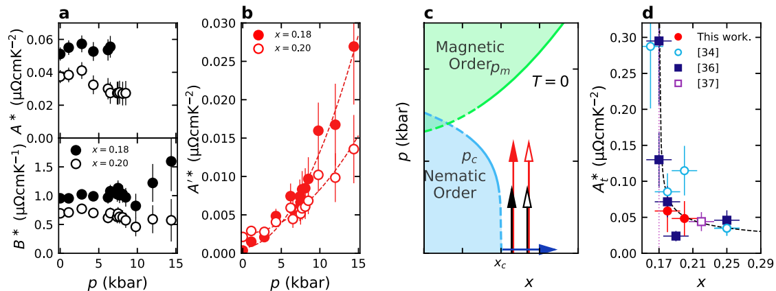
Fig. 3 Decoupled nematic and magnetic criticality in \text{FeSe}_{1-x}\text{S}_x . a Renormalized A^* coefficient (upper) and similarly renormalized B^* coefficient (lower) as a function of pressure having rescaled A and B respectively by the pressure-induced change in \rho_0 . b Similarly renormalized A^* coefficient as a function of pressure. c Schematic T = 0 phase diagram in the p - x plane showing the nematic and magnetic phase boundaries. Vertical arrows indicate the pressure-induced approach of the two studied samples to the magnetic quantum critical point and the pressure ranges over which A and A^* can be determined. The horizontal arrow represents tuning away from the nematic quantum critical point (NQCP) with increasing x (relevant to panel d ). Near x = x_c , the nematic phase boundary is shown as a dashed line to reflect its putative weak first-order nature. d Variation of A_t^* , the total low-temperature T^2 coefficient at ambient pressure rescaled by the relative growth in the carrier density, and x beyond the nematic quantum critical point near x_c \sim 0.17 (red dotted line) with data from this work and literature sources 33,36,37 . The error bars represent the estimated uncertainty in both x and the reported coefficients. We have estimated the error in the values reported in this work to be 50% due to the constraints on sample size in a pressure cell and 30% elsewhere. The uncertainty in x has been assumed to be \pm 0.015 and representative of the typical variation in x within an individual batch of samples 12 . See Supplementary Note 1 for details of the rescaling procedure. The dashed line is a guide to the eye.
