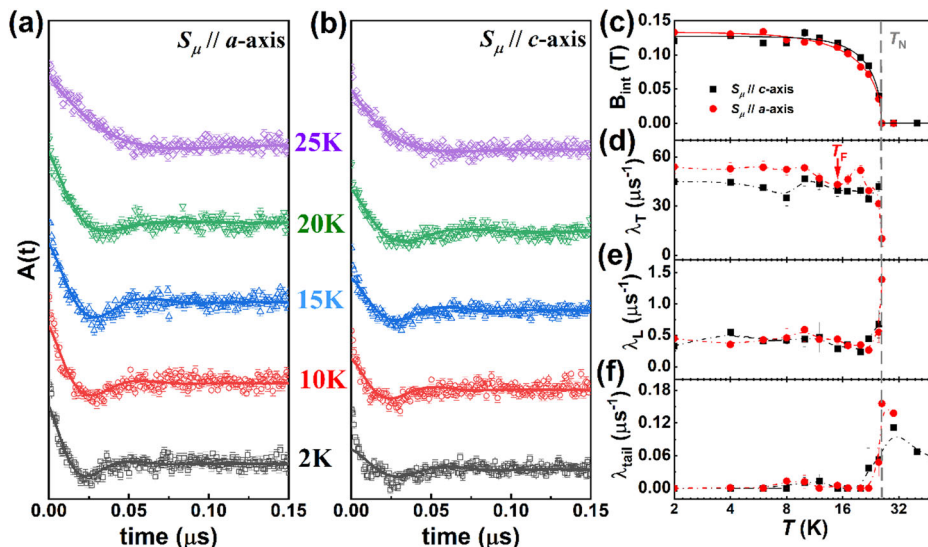
Fig. 4 | Zero-field \mu SR spectra of NCTO. a, b Zero-field (ZF) \mu SR time spectra measured at selected temperatures (displaced vertically for clarity) with the muon-spin direction S_\mu // a and c -axis, respectively. Data were taken on the M20D channel at TRIUMF. The error bars are the standard error of the mean. The solid curves represent fits to Eq. (2). c–f Temperature dependence of the B_{\text{int}} , \lambda_T , \lambda_L , and \lambda_{\text{tail}} , respectively, as derived from the analysis of ZF- \mu SR. The error bars represent the standard deviation of the fit parameters. The magnetic ordering temperature is T_N \approx 26 K and is consistent with magnetic susceptibility data. Solid lines in panels (c) are fits using a phenomenological equation described in the text; dash-dotted lines in panels (d–f) are guides to the eyes.
