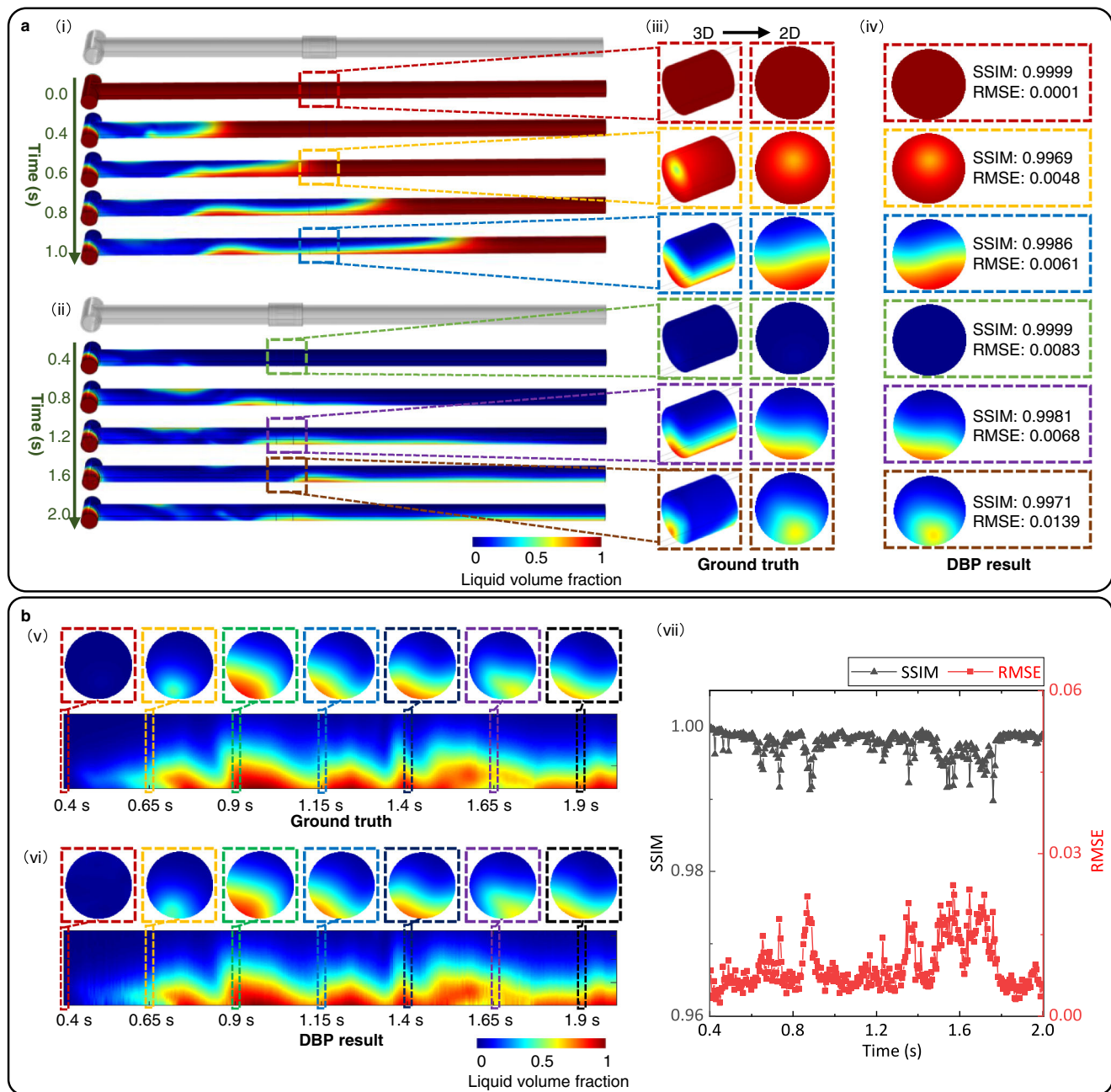
Fig. 3 Quantitative imaging of virtual gas-liquid flows by Deep Back Projection (DBP) with 50 dB Signal-to-Noise Ratio (SNR). a Two representative sets of sequential gas-liquid flows generated by three-dimensional Fluid-Electrostatic field Coupling Model (3D-FECM) and corresponding image reconstruction results of DBP. For the sequential gas-liquid flows in (i), the pipe is initially filled with liquid. For the sequential gas-liquid flows in (ii), the pipe is initially filled with gas. 3D dynamic liquid phase distributions in the ECT sensing region can be converted to the 2D volume-averaged liquid phase distributions as the ground truth (see (iii)). The cross-section images reconstructed by DBP for the gas-liquid flows in (iii) are presented in (iv). b Quantitative imaging of virtual gas-liquid transient flow with high temporal resolution (200 frames per second). (v) The authentic liquid phase distributions for evaluating the performance of image reconstruction. (vi) The images reconstructed by DBP for the gas-liquid flows in (v). The cross-section images in (vi) are a set of representative images selected from the continuous reconstruction results. (vii) The Structural Similarity Index Measure (SSIM) and Root Mean Square Error (RMSE) of the DBP results in (vi).
