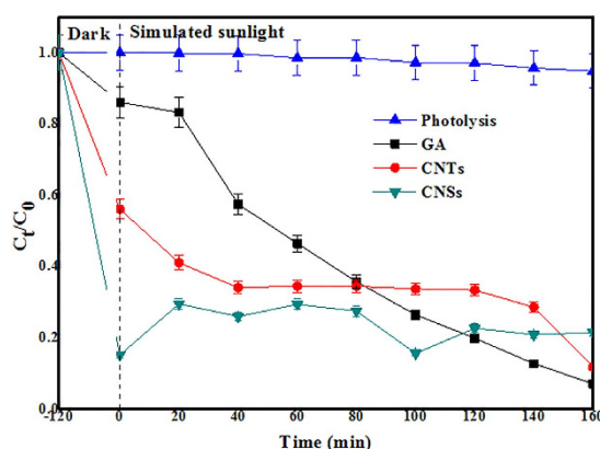
Figure 9. Degradation of 2-CP by photolysis and photocatalysis.
