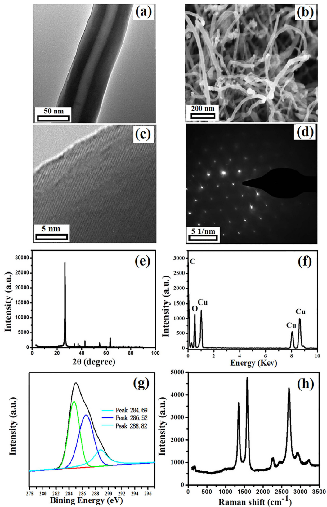
Figure 1. Characterization of the prepared CNTs from grasses: (a) TEM image, (b) SEM image, (c) HR-TEM image, (d) SAD pattern, (e) XRD pattern, (f) EDS pattern, (g) XPS pattern, and (h) Raman spectrum pattern.
