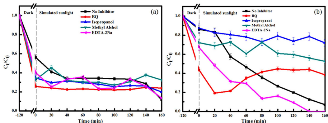
Figure 10. Plotted degradation curves of: (a) the CNTs and (b) the GA for 2-CP with additions of scavenger.
