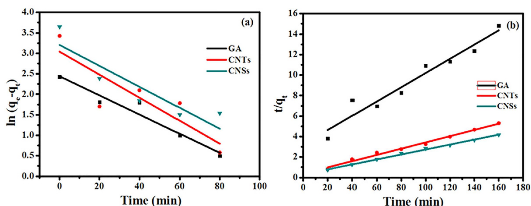
Figure 7. Adsorption kinetics of the CNMs for 2-CP: (a) pseudo-first-order kinetics, (b) pseudo-second-order kinetics.
