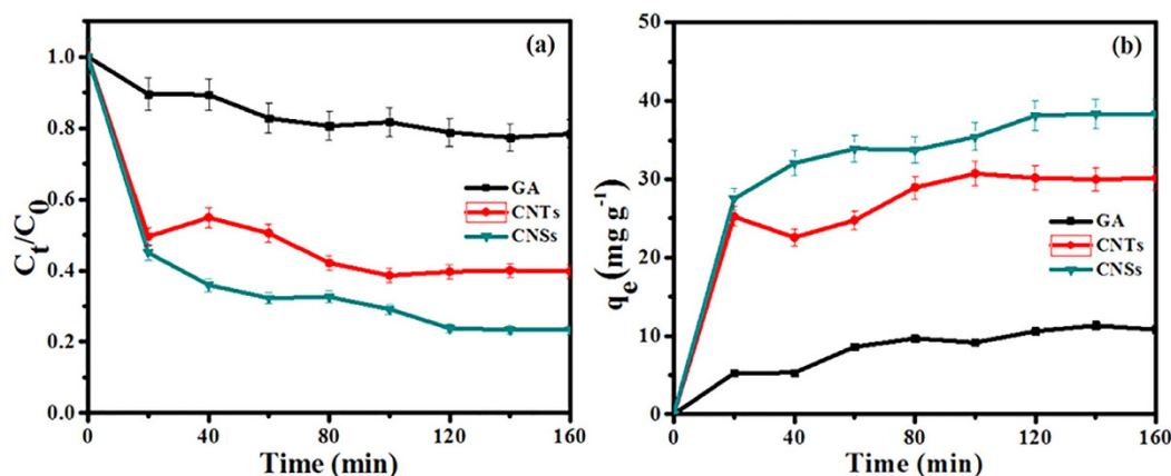
Figure 5. Adsorption equilibrium time of the CNMs for 2-CP: (a) efficiencies, (b) capacities.
