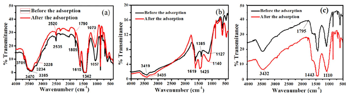
Figure 6. FTIR spectra of the CNTs, GA, and CNSs before and after the adsorption of 2-CP.
