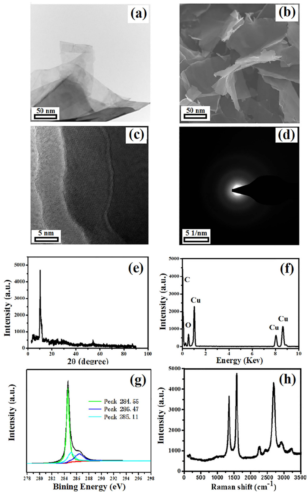
Figure 2. Characterization of the prepared GA from grasses: (a) TEM image, (b) SEM image, (c) HR-TEM image, (d) SAD pattern, (e) XRD pattern, (f) EDS pattern, (g) XPS pattern, and (h) Raman spectrum pattern.
