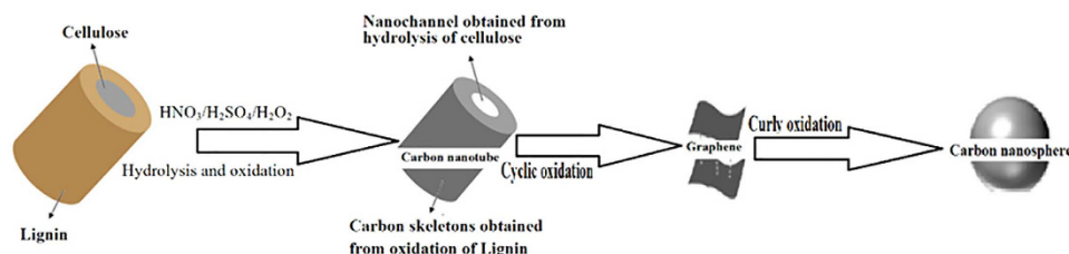
Figure 4. Formation schematic of the CNMs from grasses.
