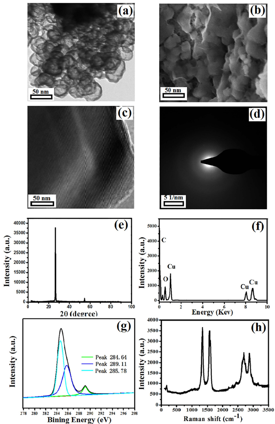
Figure 3. Characterization of the prepared CNSs from grasses: (a) TEM image, (b) SEM image, (c) HR-TEM image, (d) SAD pattern, (e) XRD pattern, (f) EDS pattern, (g) XPS pattern, and (h) Raman spectrum pattern.
