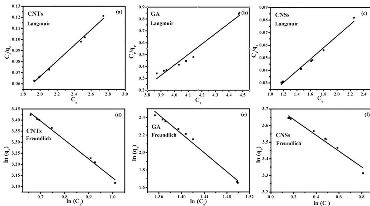
Figure 8. Adsorption isotherms of the CNMs for 2-CP: (a–c) Langmuir isotherm of the CNTs, GA, and CNSs, (d–f) Freundlich isotherm of the CNTs, GA, and CNSs.
