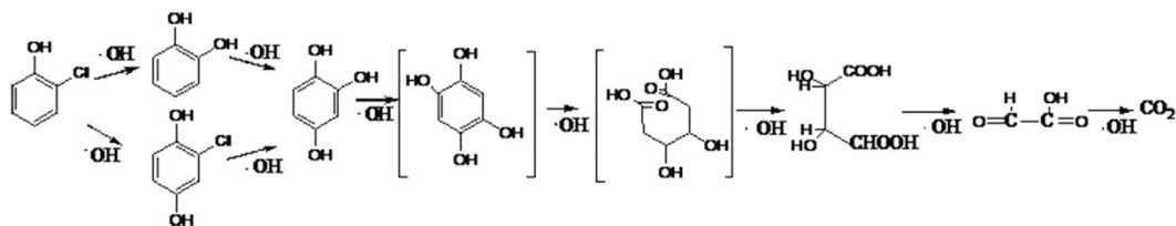
Figure 11. Possible reaction pathway involving \cdot\text{OH} radicals.
